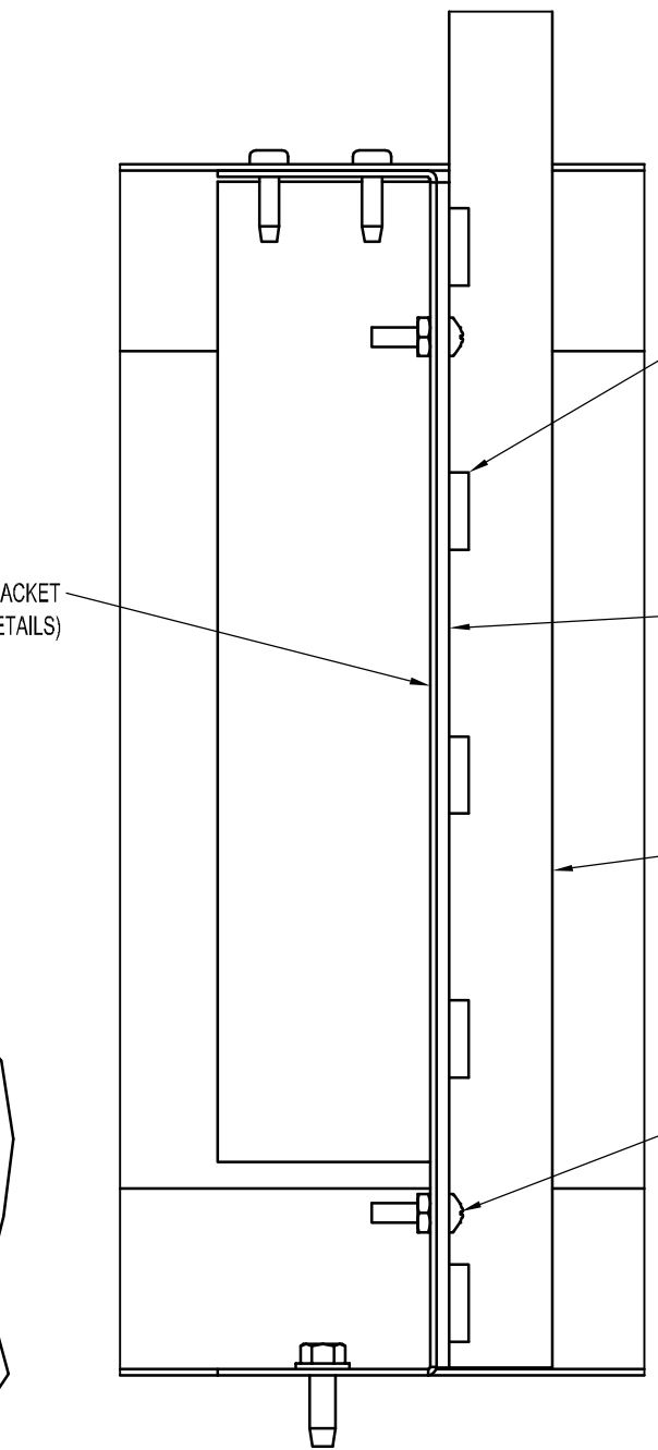
MOUNTING BRACKET SIDE VIEW SCALE 1/2" = 1"
